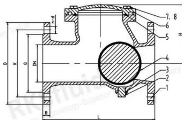
DN200-DN500
