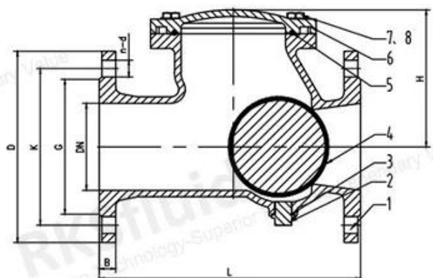
DN200-DN500
