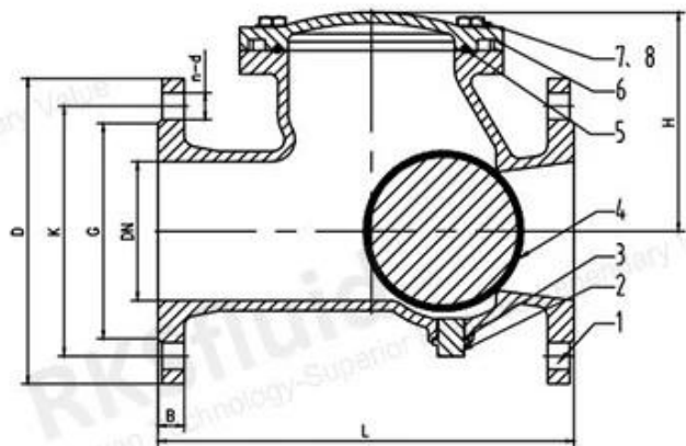
DN200–DN500
