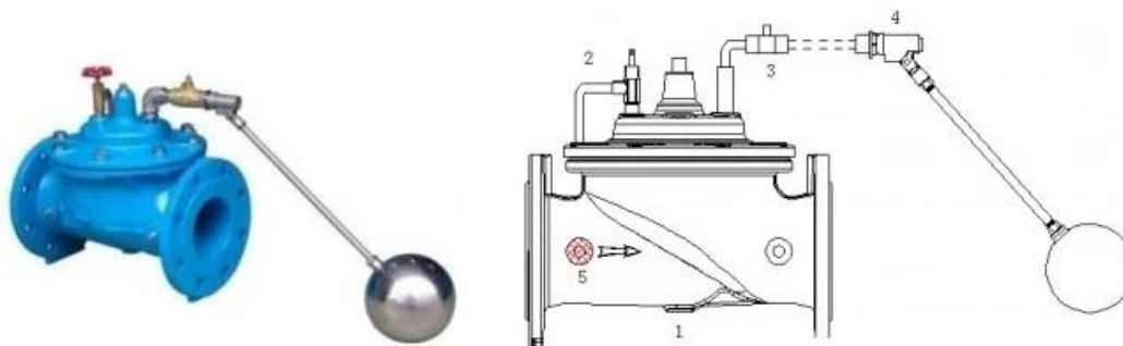
1. Main valve 2. Needle valve 3. Ball valve 4. Float pilot 5. Strainer
