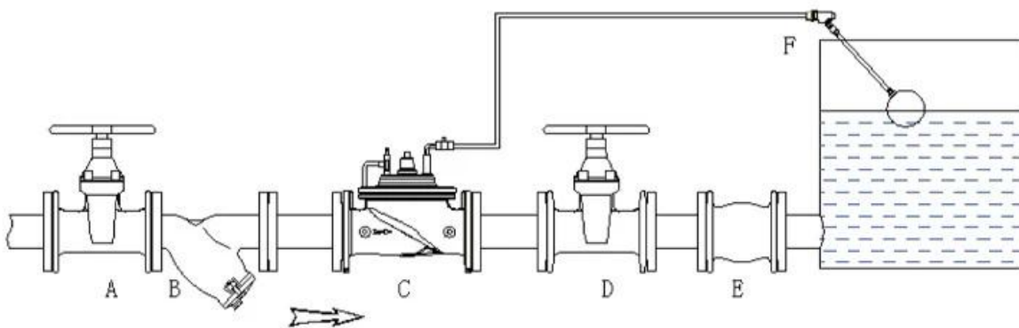
A. Shut off valve F. Float pilot B. Y strainer C. Float control valve D. Shut off valve E. Soft joint
